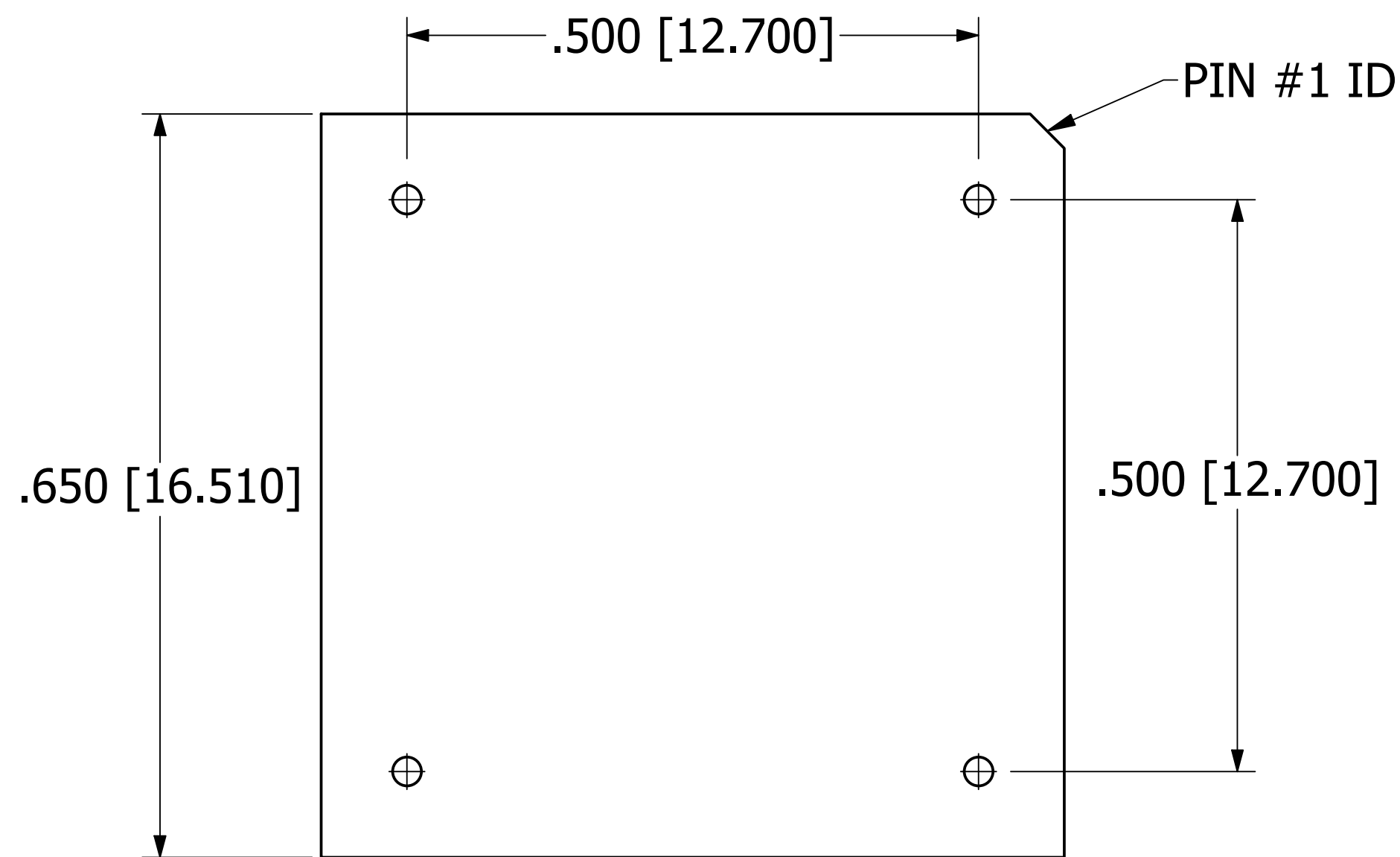
BOTTOM VIEW
